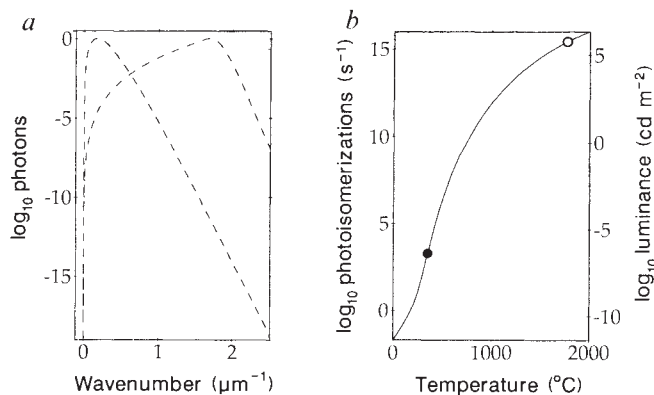
Fig. 1 a , The dashed line is the spectral photon radiance N_{e\lambda}(T, \lambda) of 350 °C black-body radiation as a function of wavenumber, 1/\lambda . The dotted line is the quantum efficiency \alpha(\lambda) of rhodopsin. The dotted-and-dashed line is the product N_{e\lambda}(T, \lambda)\alpha(\lambda) . All three plots are relative to their maximum values. b , The number of photoisomerizations per second N_a(T) in the shrimp eye (left-hand scale, assuming \omega = \pi/2 ) and the luminance L'(T) (right-hand scale) as a function of the temperature of the black-body radiator. At 350 °C (●) the shrimp eye absorbs 1,800 photons per second under optimal conditions and the luminance is 0.43 \times 10^{-6} \text{ cd m}^{-2} . The open symbol (○) is explained below.
